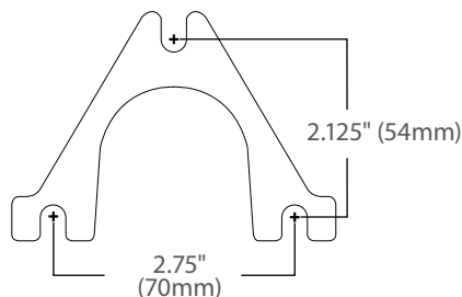
Wall Mount
